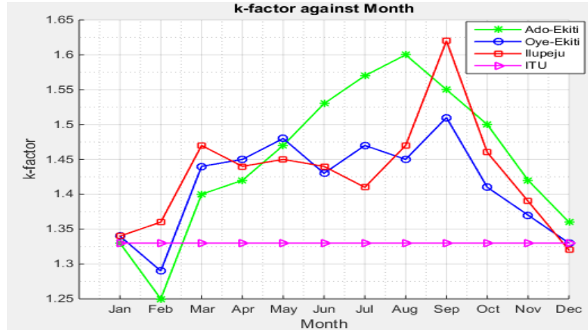
Figure 3: Variation of effective earth radius with months for Ekiti State environment
