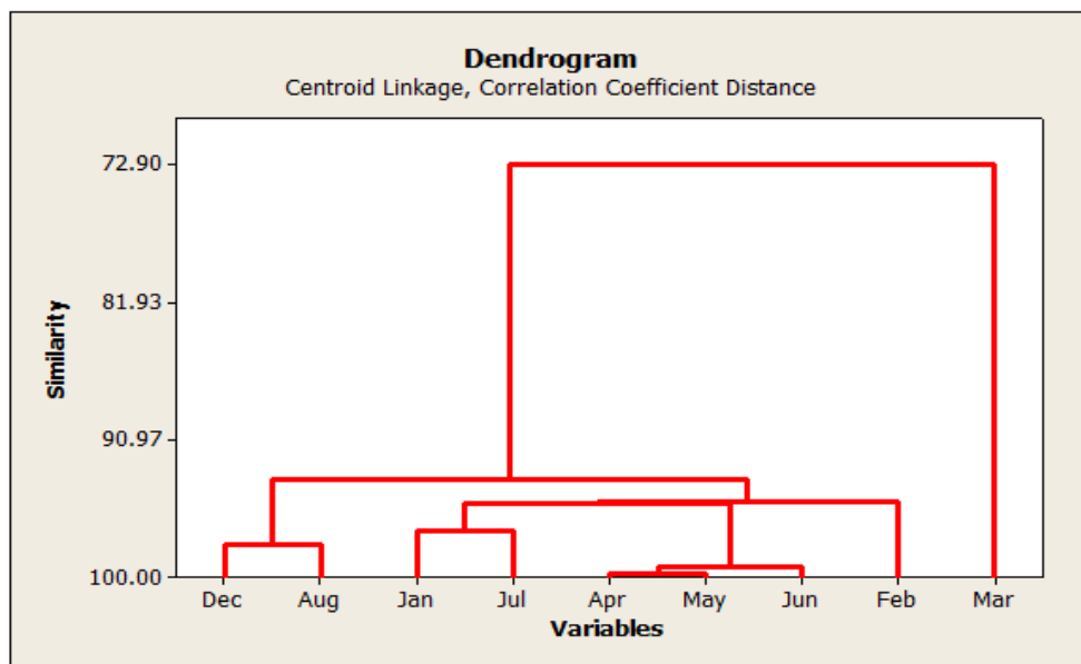
Fig 3: Dendrogramme Showing the Clusters
